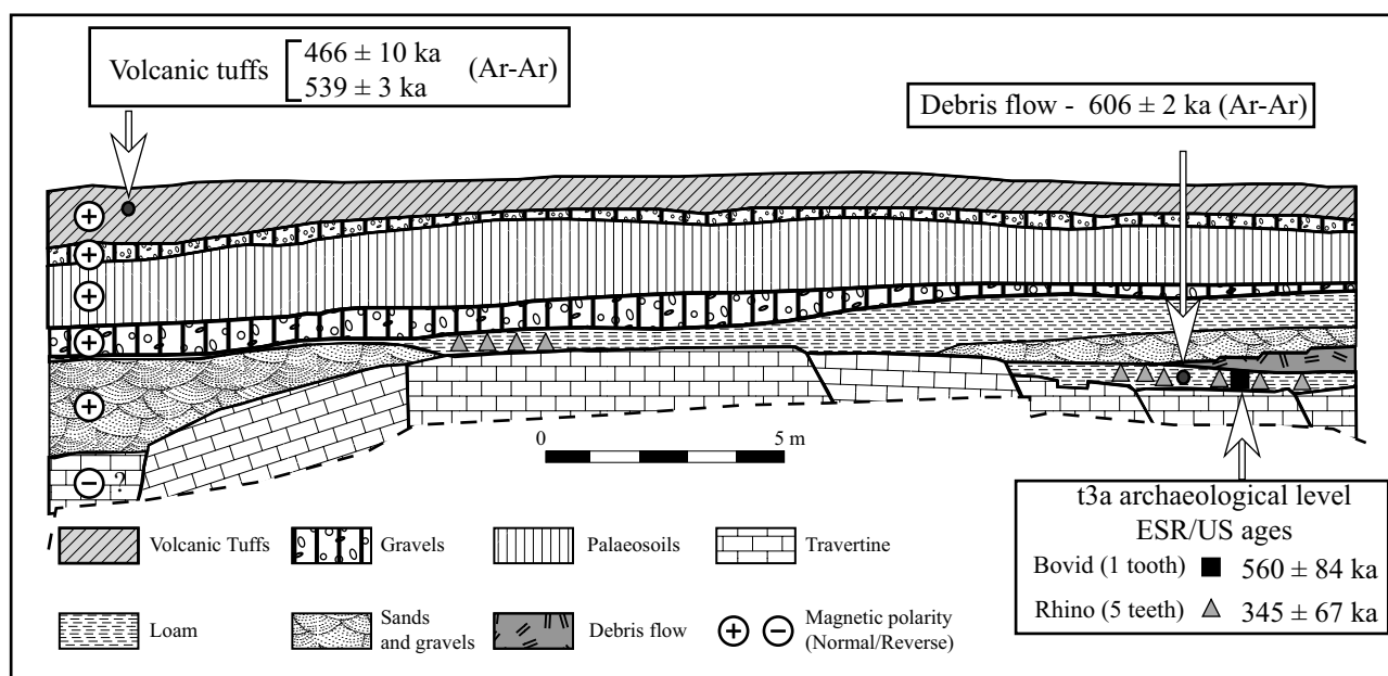
Fig. 7: ESR/U-series ages obtained on teeth recovered from the Isernia la Pineta Site, Italy (after Perretto et al. , 1983).
