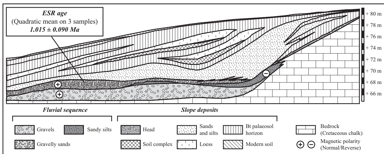
Fig. 5: ESR ages obtained on sediments and ESR/U-series age derived from a bovid tooth sampled in the fluvial deposits of the Grèce-Autoroute Terrace, Somme Valley, France (from a geological section by courtesy of P. Antoine).
